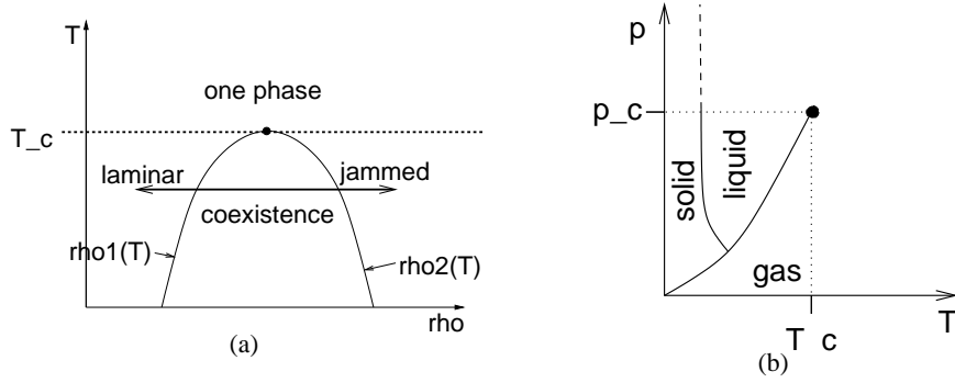
Fig. 2. (a) Phase diagram of the gas-fluid model as a function of the density and the temperature T . (b) “Standard” pressure-temperature (PT) diagram with critical point. For T > T_c or p > p_c , there is no gas-liquid transition any more. In that case, distinguishing between liquid and gas phases does not really make sense.
