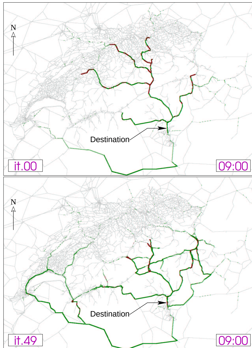
FIGURE 2: Example of Relaxation Due to Feedback. TOP: Iteration 0 at 9:00 – all travelers assume the network is empty. BOTTOM: Iteration 49 at 9:00 – travelers take more varied routes to try to avoid one another. Red (dark gray in b/w version) indicates jams, green (dark gray in b/w version) indicates free-flowing traffic, and gray indicates empty roads.
