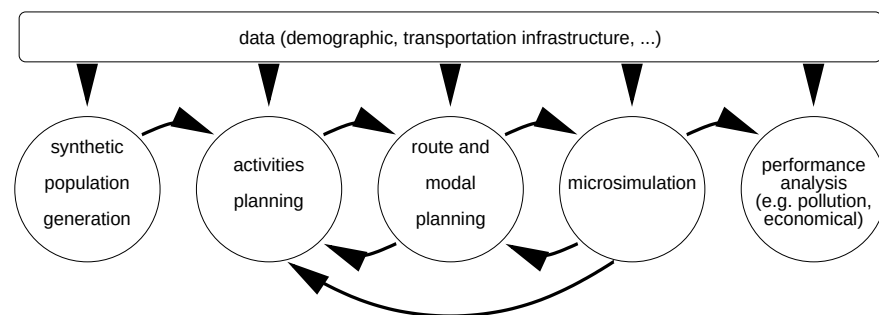
FIGURE 1: TRANSIMS Modules
