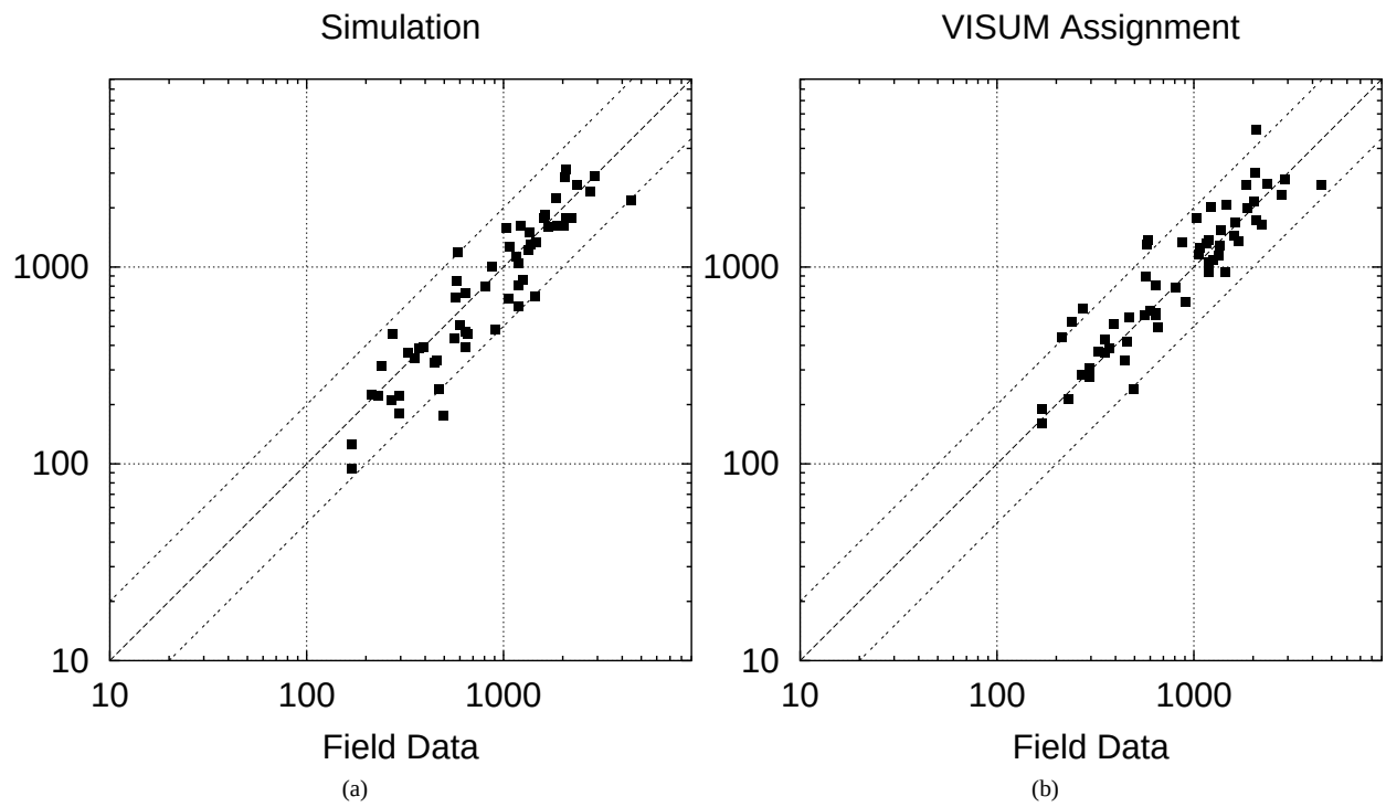
FIGURE 4: Comparison to Field Data. (a) Simulation vs. field data for the 50th iteration. The x-axis shows the hourly counts between 7am and 8am from the field data; the y-axis shows throughput on the corresponding link from the simulation. (b) VISUM assignment vs. field data. The x-axis is the same as (a); the y-axis shows the volume obtained from the assignment model.
