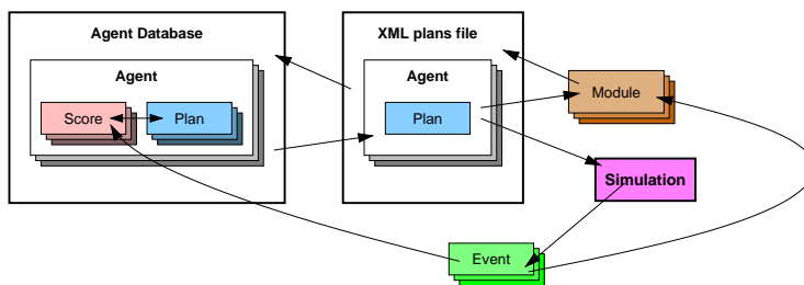
Figure 3: Components and data flow in the framework
