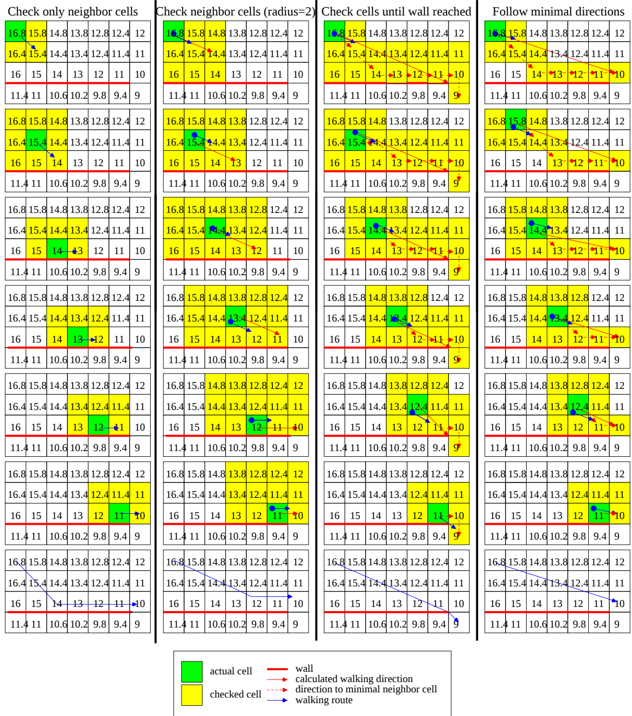
Figure 2: Different algorithms to calculate the desired velocity (walking direction) from a given potential field.
