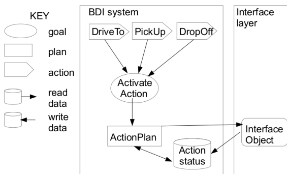
Figure 6. Generic Action Goal and Plan structure
