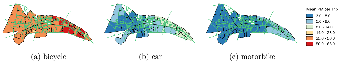
Figure 4: A comparison of inhaled PM 2.5 per trip (in \mu g/km ) for different modes on 22 Nov. 2017.
