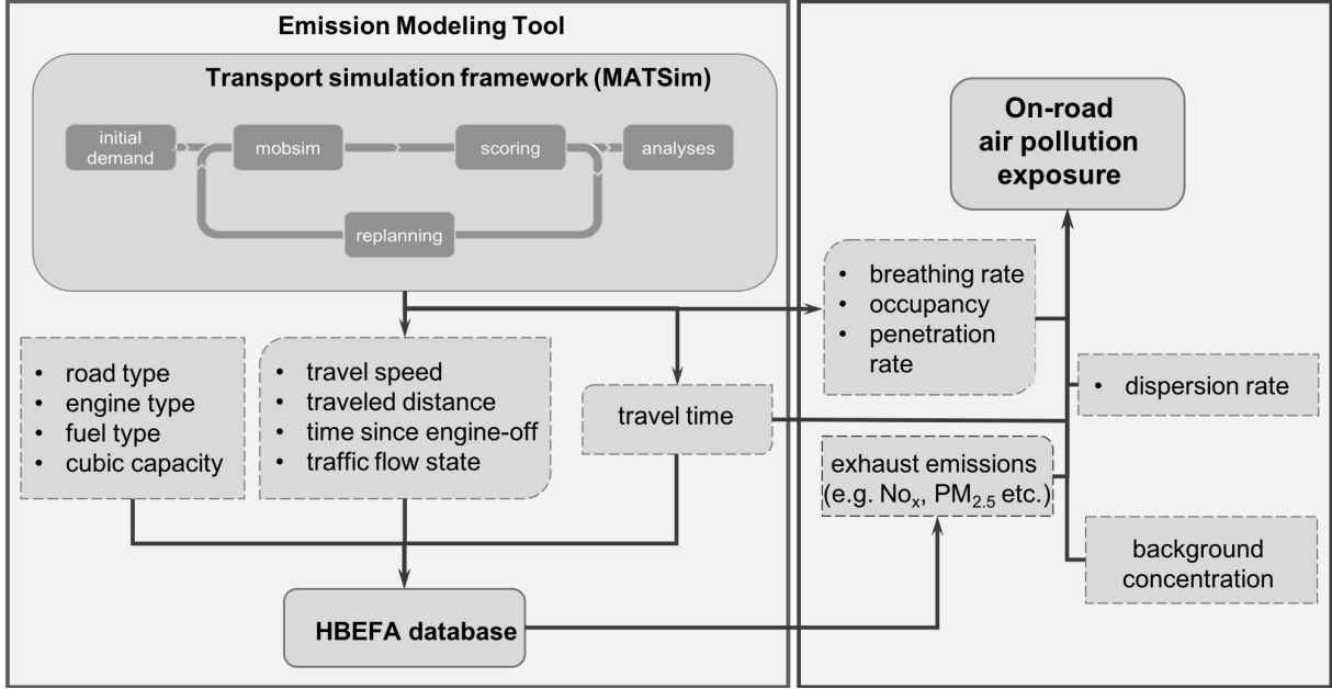
Figure 1: Integration of MATSim controller and emission modeling tool with on-road air pollution exposure
