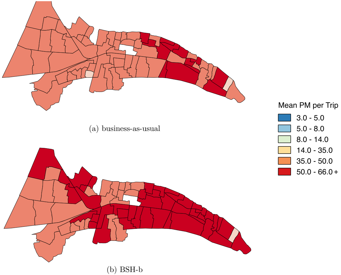
Figure 6: Mean PM 2.5 ( \mu\text{g}/\text{km} ) per trip for cyclists in business-as-usual and BSH-b scenarios
