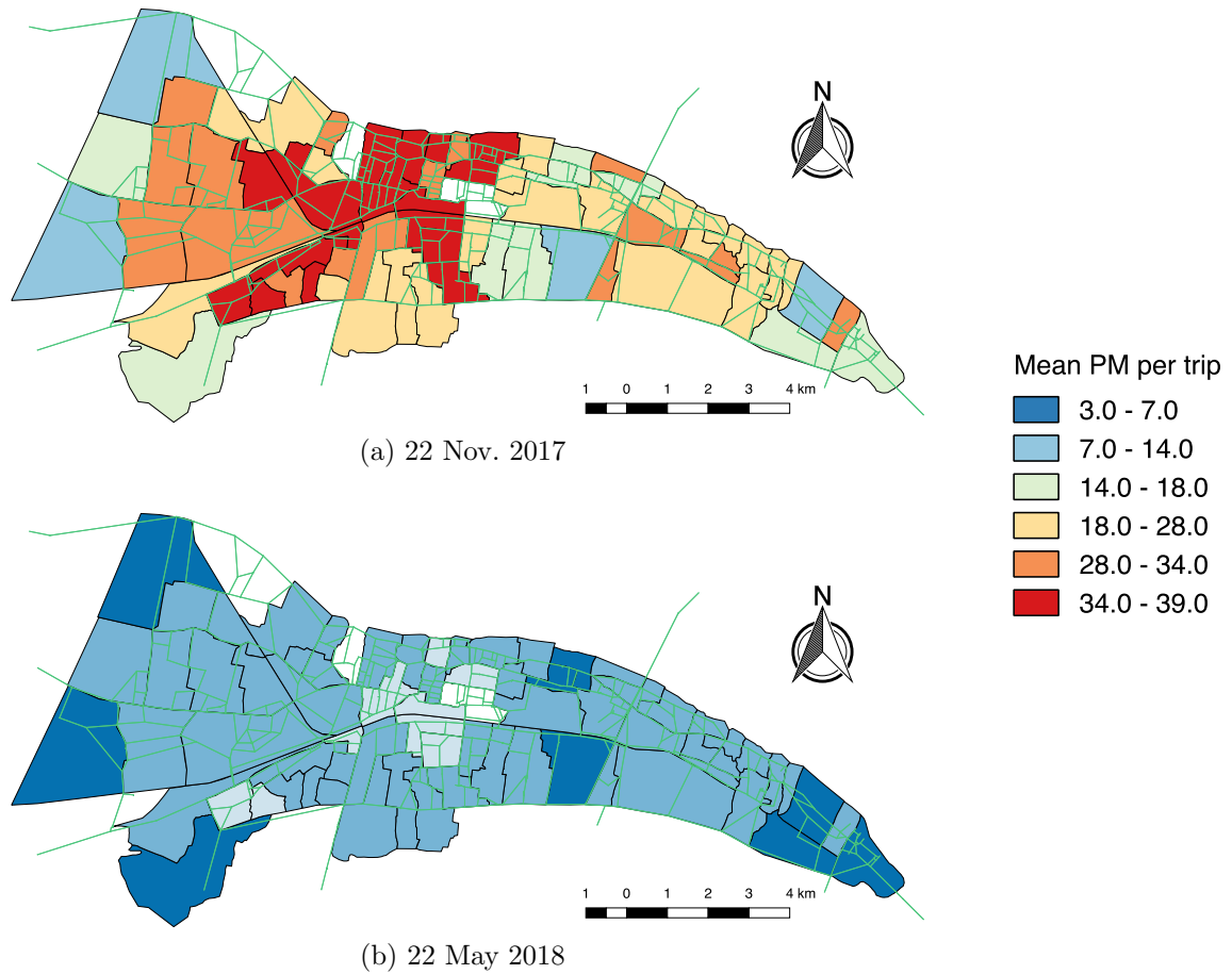
Figure 3: Mean PM 2.5 ( \mu g/km ) per trip for different days
