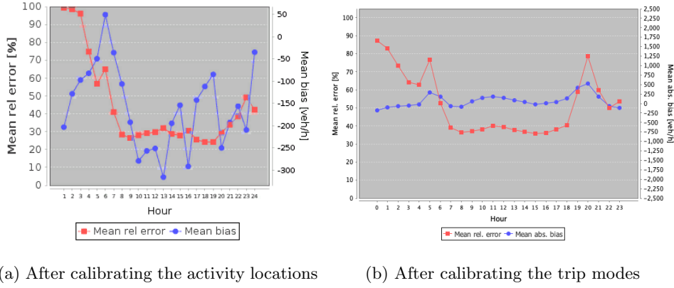
Figure 1: Evaluation of traffic counts match after the first and second calibration step.
